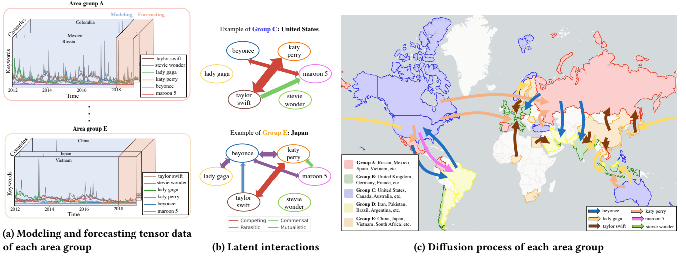
Figure 1: Modeling power of FLUXCUBE for online user activity data related to six artists (World#1): (a) Given the original data (gray lines), FLUXCUBE captures the dynamics of social activities (blue). Furthermore, FLUXCUBE provides a multiple steps ahead forecast (red). (b) Our method detects the hidden interactions between keywords in any country. The arrows indicate the direction and the type of influence. (c) It also automatically discovers similar area groups based on their keyword interactions and then finds the flow of influence of each keyword between area groups. The figure visualizes the flow of influence in 2015.
