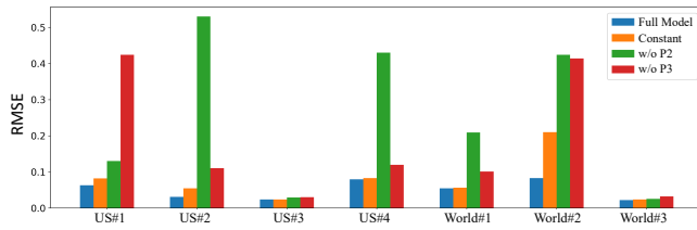
Figure 4: Experimental ablation results for RMSE performance of 52 weeks ahead forecasting.
