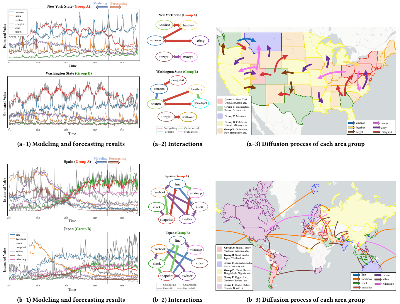
Figure 5: FLUXCUBE modeling and forecasting results for US#1 (a) and World#2 (b) data: (a/b-1) shows the modeling and forecasting results of FLUXCUBE given the observational data. It represents observational data in gray and the modeling and forecasting results for each keyword in various colors. (a/b-2) shows the network graphs summarizing four latent interactions between keywords in each country. FLUXCUBE uncovers four types of interaction, each of which is represented by arrows. Competing and mutualistic relationships are bidirectional, while commensal and parasitic relationships are one-directional: source species benefit from destination species' growth. (a/b-3) shows the clustering results with countries/states divided into multiple area groups and the flow of influences between each area group.
