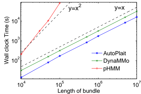
Figure 9: AUTOPLAIT scales linearly: wall clock time vs. dataseize n . Our method and DynaMMo are linear (i.e., slope = 1 in log-log scale), while pHMM is at least quadratic (i.e., slope \approx 2 ). AUTOPLAIT is 472 times faster than pHMM at n = 10^5 .
