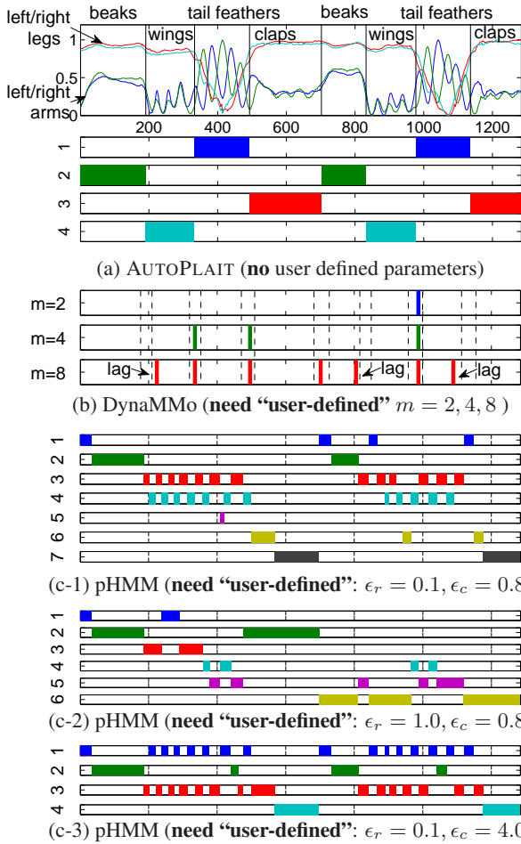
Figure 6: AUTOPLAIT is fully automatic: it finds the right cuts automatically: (a) result of AUTOPLAIT, (b) three sets of results ( r, m = 2, 4, 8 ) for DynaMMo, (c) three sets of results ( \epsilon_r = 0.1, 1.0, \epsilon_c = 0.8, 4.0 ) for pHMM. Note that AUTOPLAIT finds the correct count and location of the cuts, while its competitors are very sensitive to user-defined parameters.
