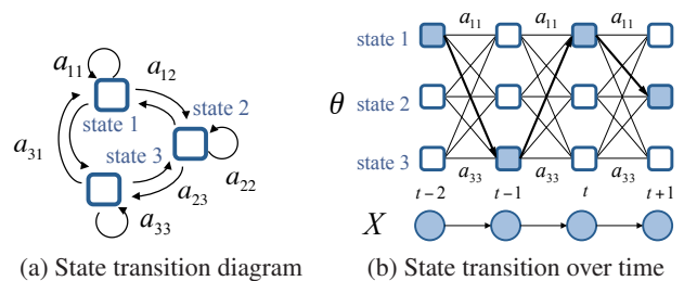
Figure 2: Illustration of the HMM structure. Given a bundle \mathbf{X} and a model \boldsymbol{\theta} (here, hidden states k = 3 , sequence length n = 4 ), the colored states in (b) denote the Viterbi path.
