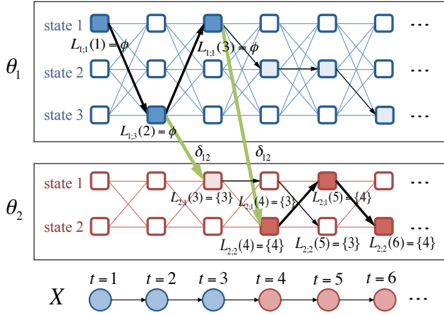
Figure 5: Illustration of CutPointSearch. Given a bundle \mathbf{X} and two models \theta_1, \theta_2 (here, duration n = 6 ), our algorithm requires only a single scan to detect the regime cut point (i.e., at time-tick t = 4 ). Note that the colored cells indicate the optimal states (i.e., Viterbi path). At time-tick t = 3 and 4 in the red regime, the algorithm finds \mathcal{L}_{2;1}(3) = \{3\} and \mathcal{L}_{2;2}(4) = \{4\} as the first and second cut-point candidates. and at time-tick t = 6 , \mathcal{L}_{2;2}(6) = \{4\} is chosen as the optimal cut point.
